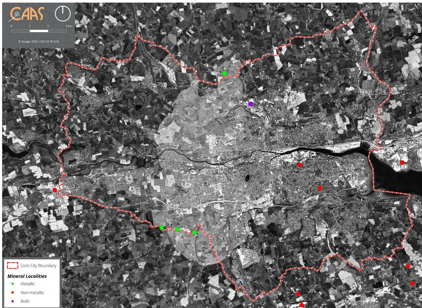
Figure 4.15 Mineral Localities
