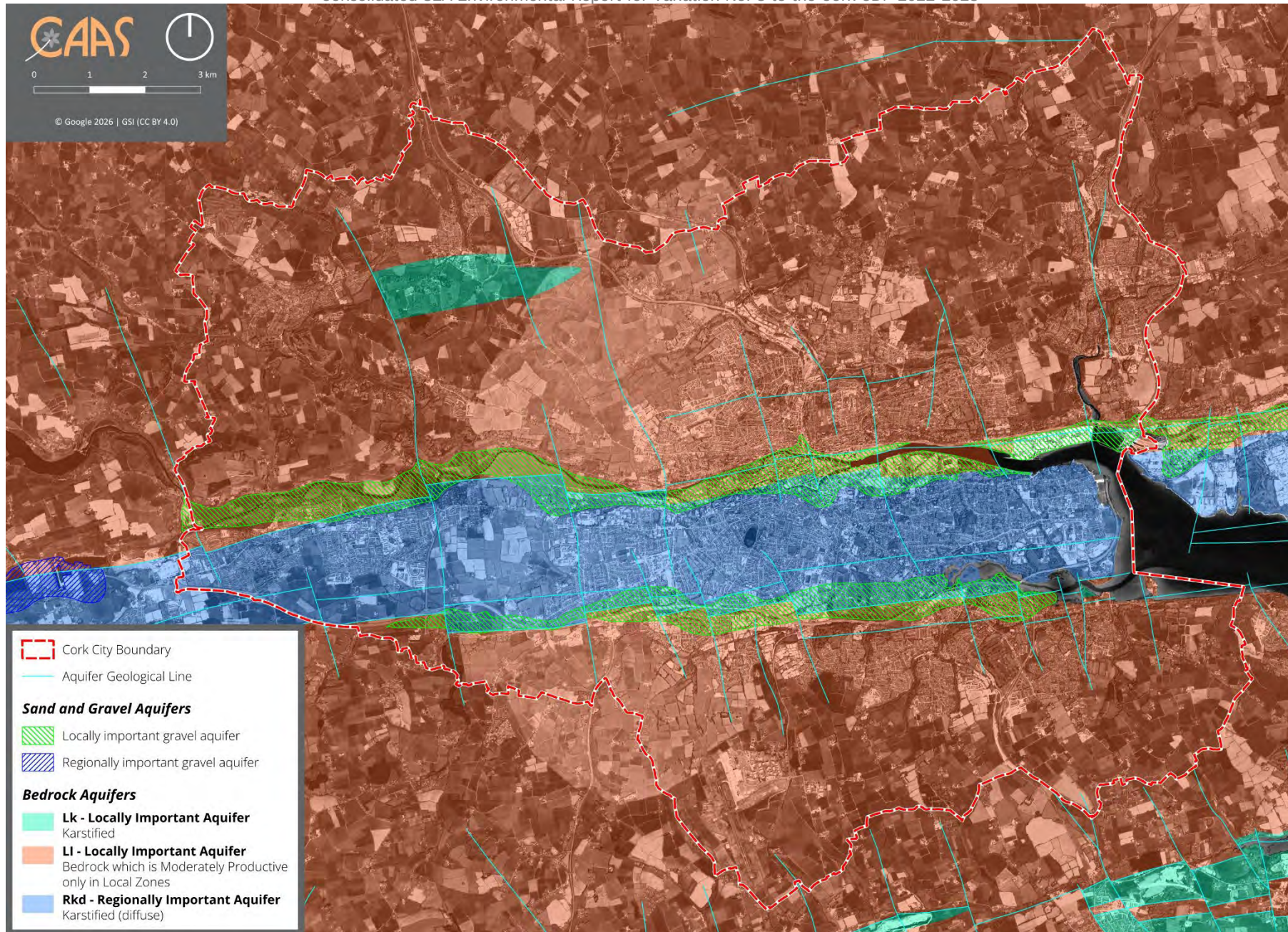
Figure 4.14 Groundwater Productivity
